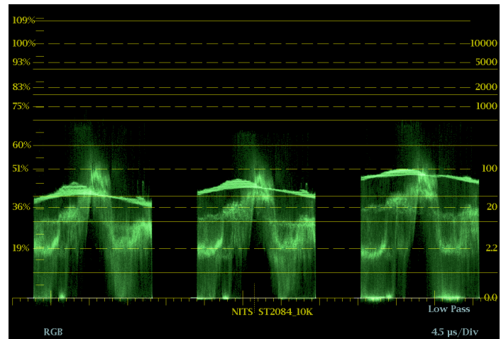
Waveform display showing HDR graticule (ST2084 10K Narrow with Nits scale)
