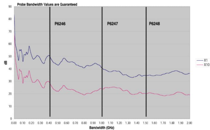
P6246/47/48 CMRR Ratio Graph
