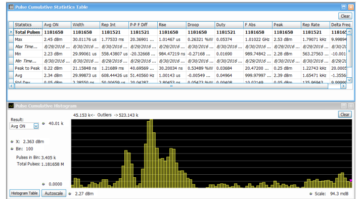
Cumulative statistics provides timestamps for Min, Max values as well as Peak to Peak, Average and Standard deviation over multiple acquisitions, further extending the analysis. Histogram shows you outliers on the right and left.
